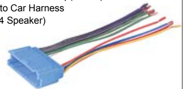
HN1072(GWS-347) General Motors 1994-Up (32 Pin)
